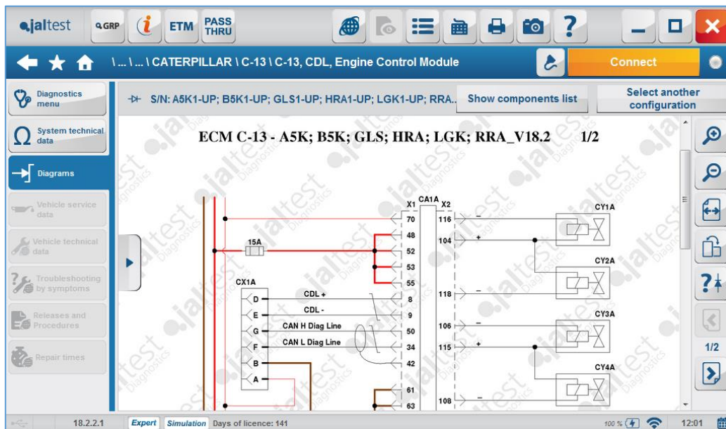
Wiring Diagram on Engine C-13
