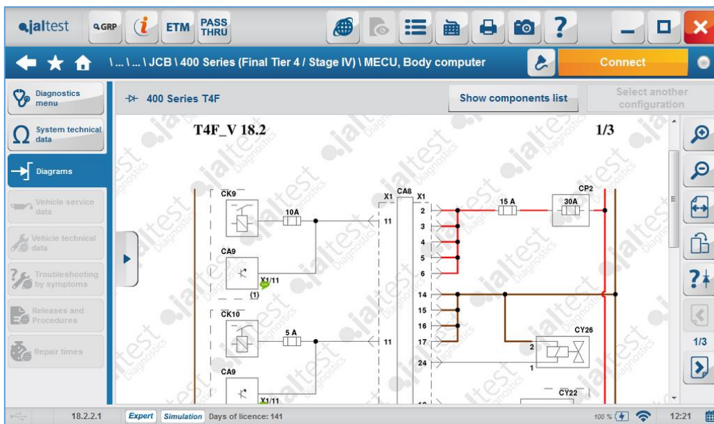
MECU Wiring Diagram JCB 400 Series (Final Tier 4/Stage IV)
