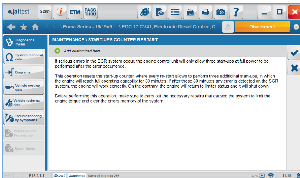
START-UPS COUNTER RESTART, EDC 17 CV41
